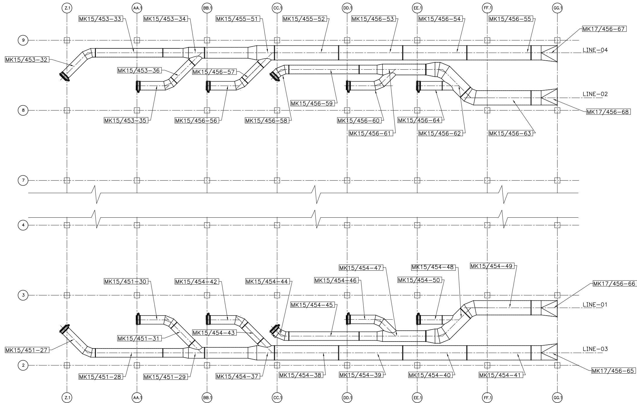
PLAN AT EL 98.00 TO 112.00
